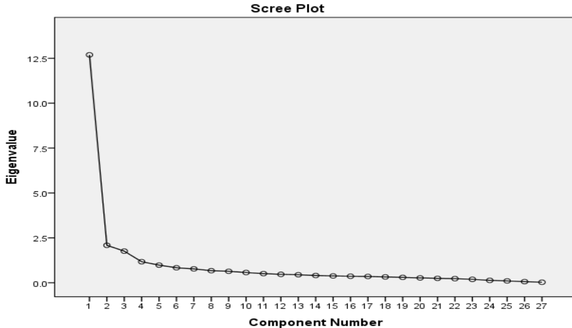
Figure 1. Scree Plot
