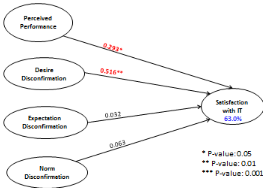
Figure 2. Results of PLS Model 2
